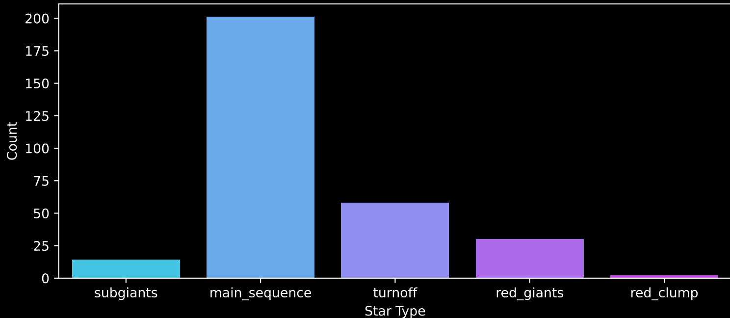
GALAH DR4 Field: [7011] Count plot of Star Type
