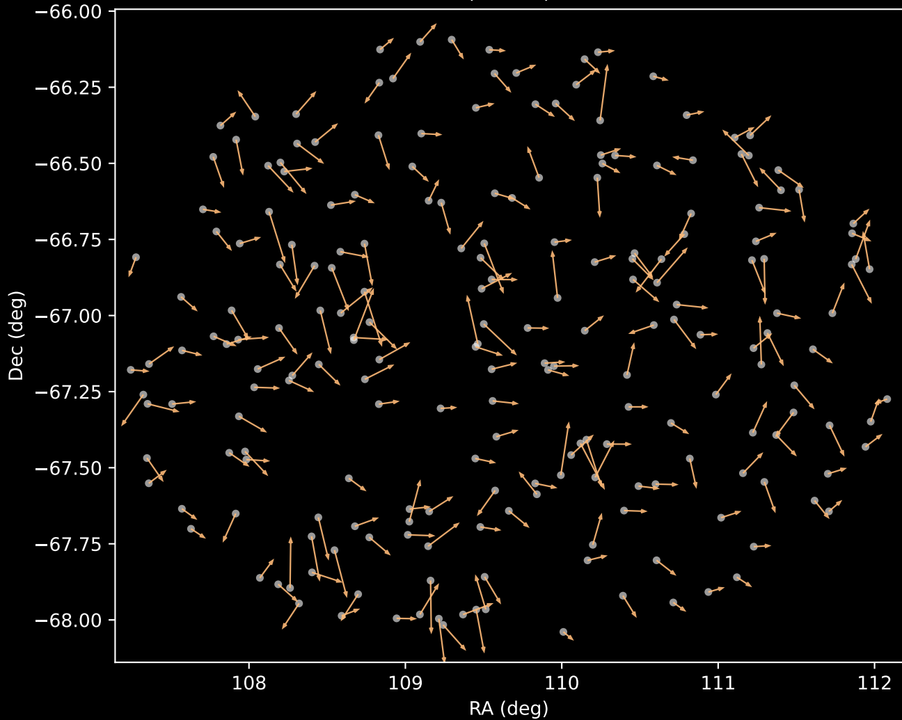
GALAH DR4 Cluster 3 Proper Motion Vectors (n=212)
