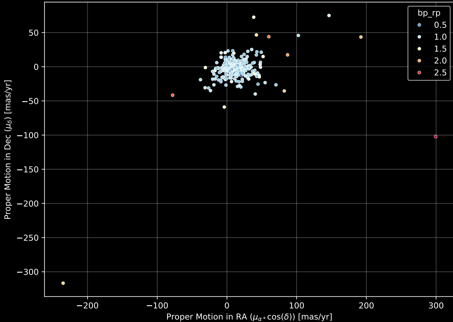
GALAH DR4 Field: [7011] Proper Motion Diagram (n= 305)
