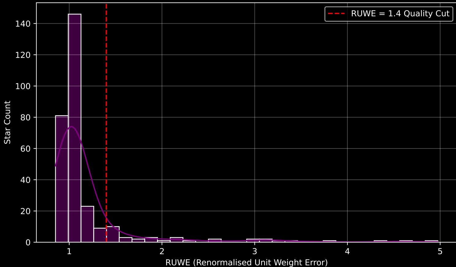
GALAH DR4 Field [7011] RUWE Distribution (n= 294)
