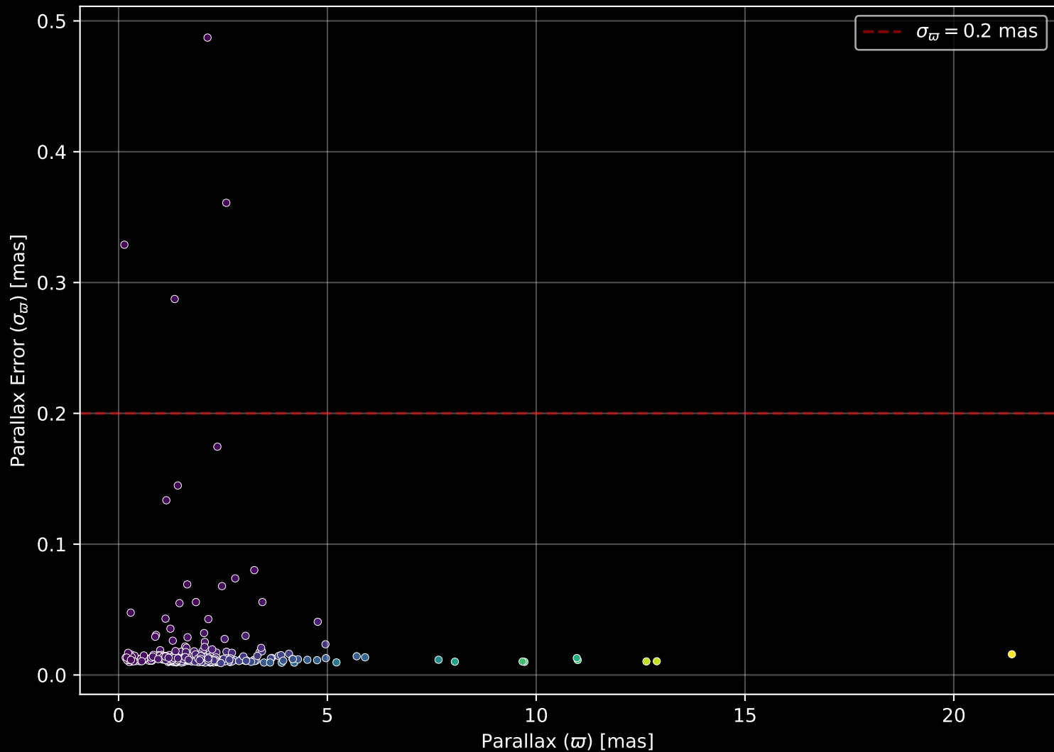
GALAH DR4 Field: [7011] Parallax Quality (n= 305)
